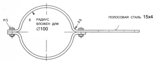
Хомут IS 100
